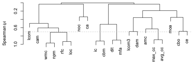
Fig. 2: Clustered factors after correlation analysis for Poi-3.0.
