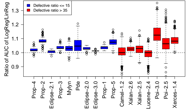
Fig. 5: Ratio of AUC of discretized/regression-based defect statistical classifiers across different datasets. The datasets are ordered based on their defective ratio from low to high.
