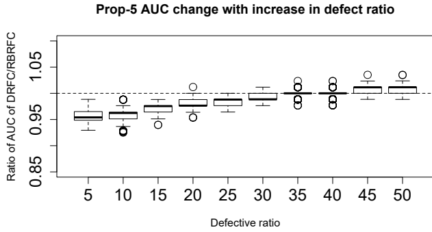
Fig. 7: Boxplot of the ratio between AUC of DRFC/ AUC of RBRFC on Prop-5.
